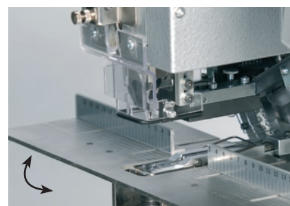
Bewegliches (aktives) Fingerschutzsystem Movable (active) finger guard system
