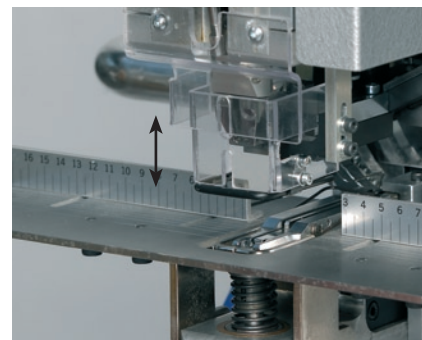
Bewegliches (aktives) Fingerschutzsystem Movable (active) finger guard system
