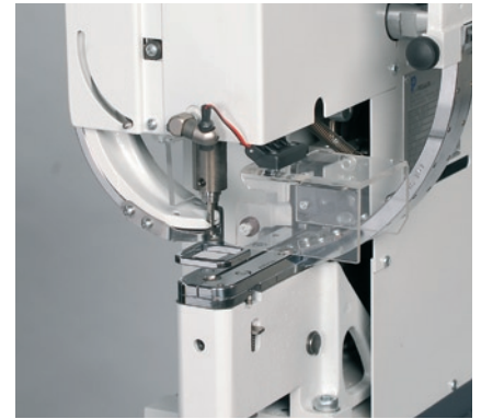
Bewegliches (aktives) Fingerschutzsystem Movable (active) finger guard system
